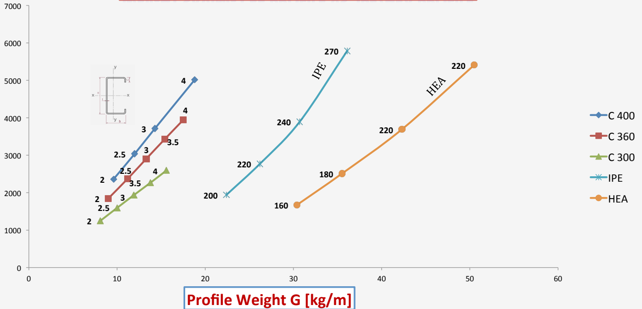
WEIGHT SAVING CEE PROFILE VS. IPE/HEA PROFILE
