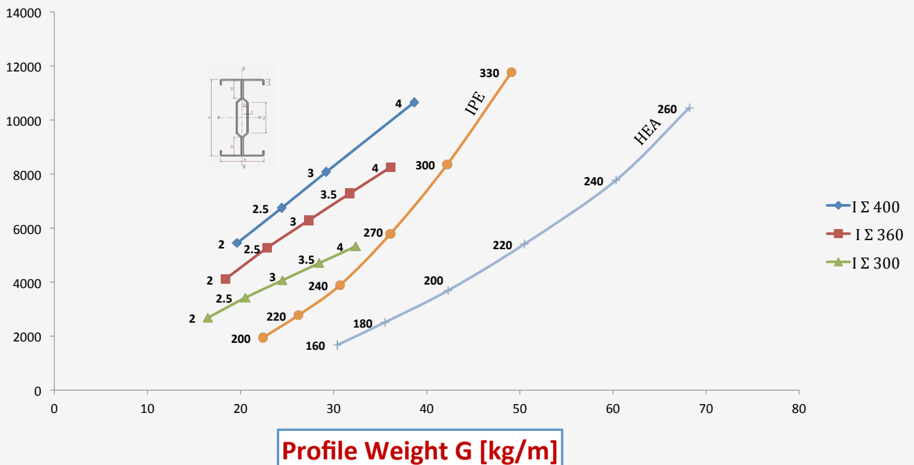
WEIGHT SAVING I SIGMA PROFILE VS. IPE/HEA PROFILE
